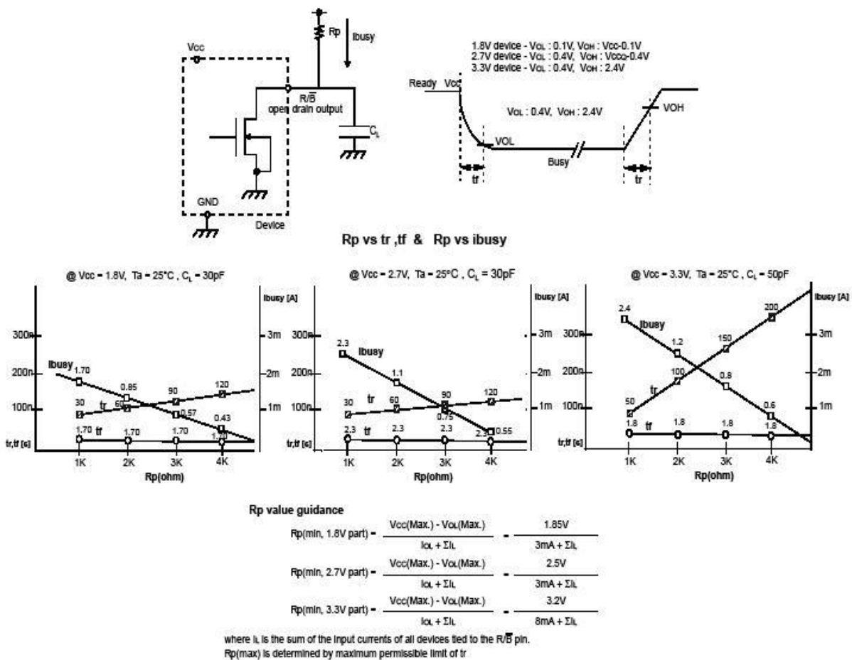
Figure 28 : Ready/Busy Pin electrical application
