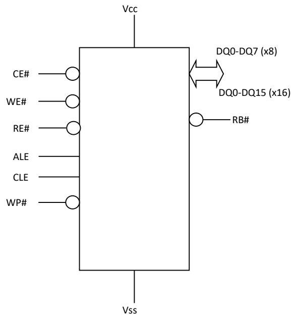
Figure 1: Logic Diagram
