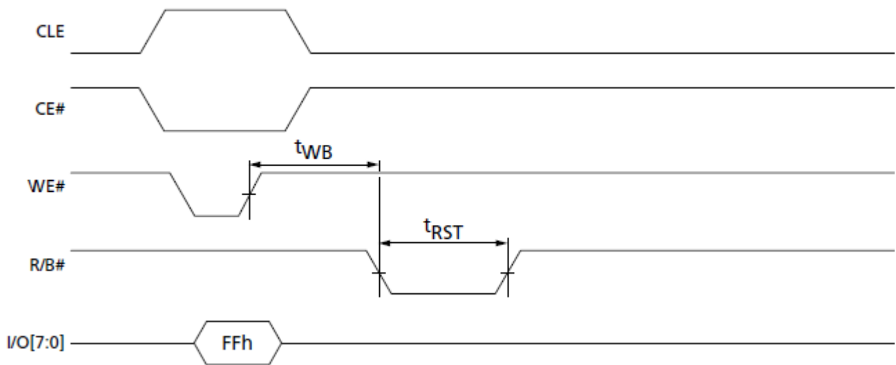
Figure 23 : Reset operation timing
