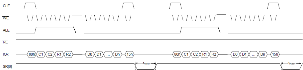
Figure 18: Cache Program Start
