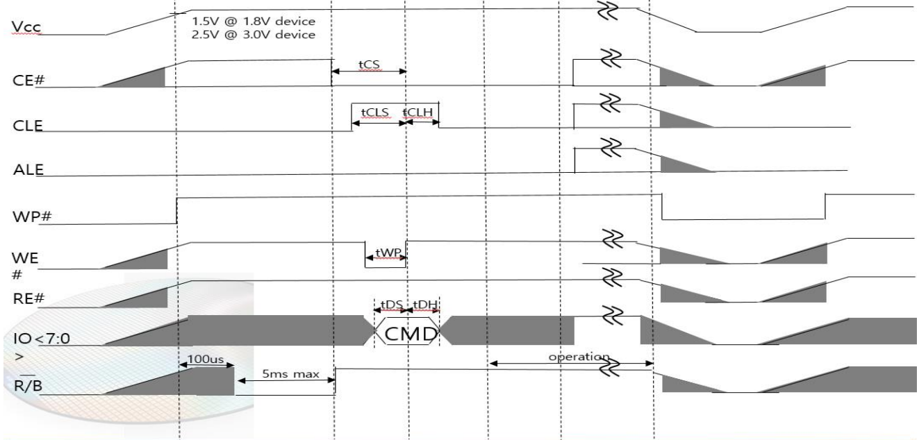
Figure 27 : power up time sequence
